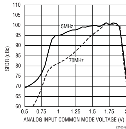
LTC2215 SFDR vs Analog Input Common Mode Voltage, 5MHz and 70MHz, -1\text{dBFS}
