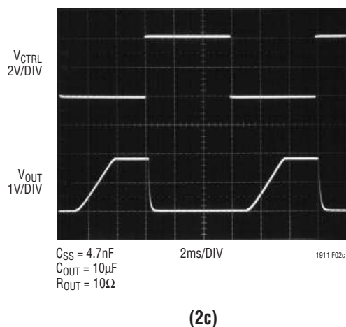
Figure 2. Shutdown/Soft-Start Operation
