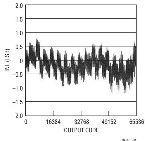
Integral Nonlinearity vs Output Code (LTC1867)
