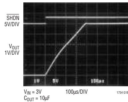
Start-Up Time
