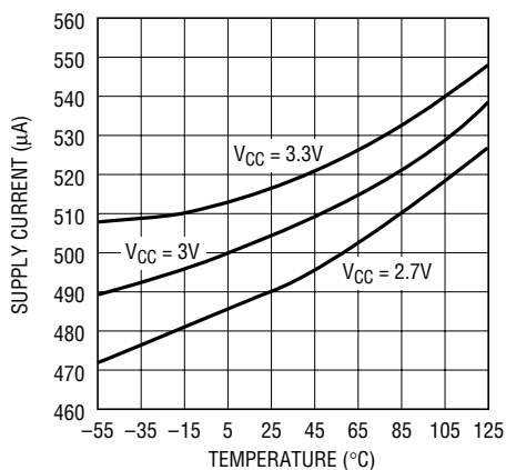
LTC1657L Supply Current vs Temperature
