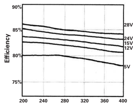
III. Efficiency vs. Input Voltage
