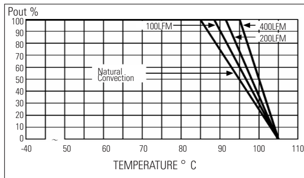
MODEL 100VFI
