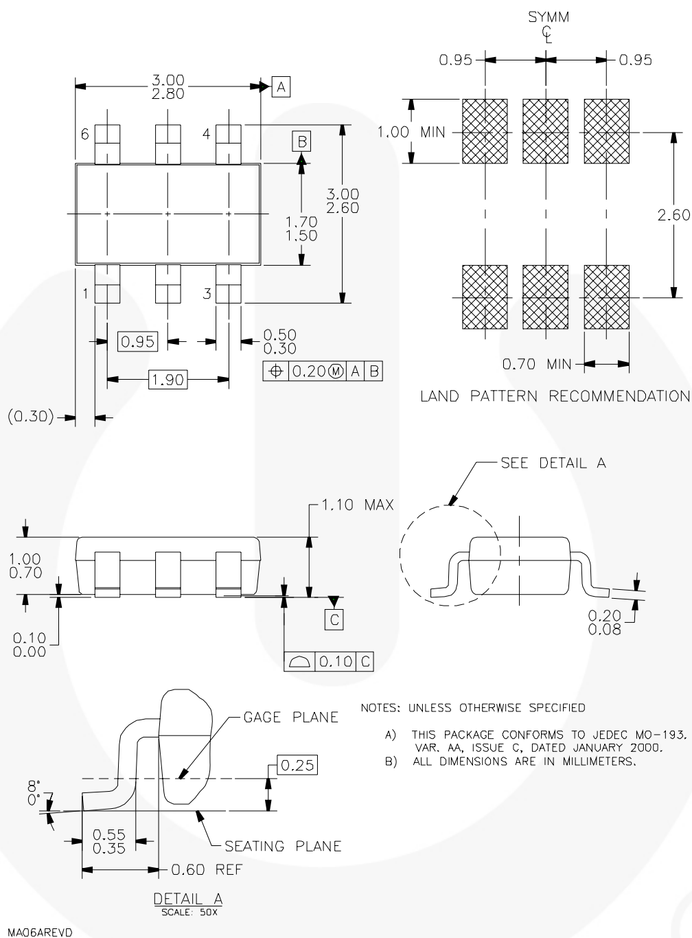
Figure 18. 6-Pin, SSOT-6 Package
