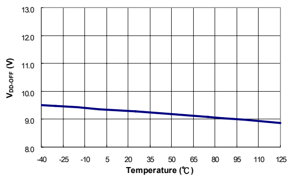
Figure 7. Turn-off Threshold Voltage ( V_{DD-ON} ) vs. Temperature
