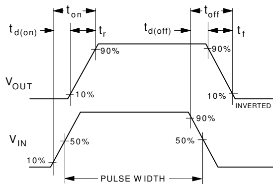
Figure 12. Switching Waveforms.
