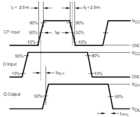
FIGURE 3. AC Waveforms
