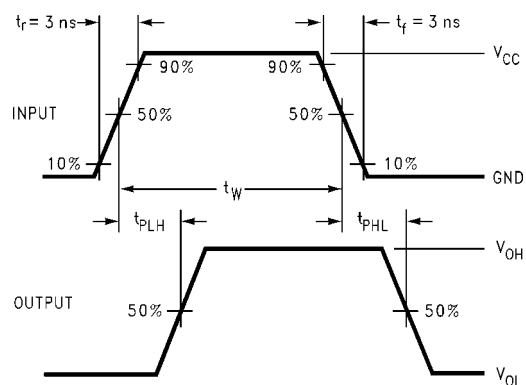
FIGURE 2. AC Waveforms
