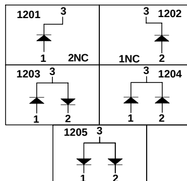
Connection Diagram
