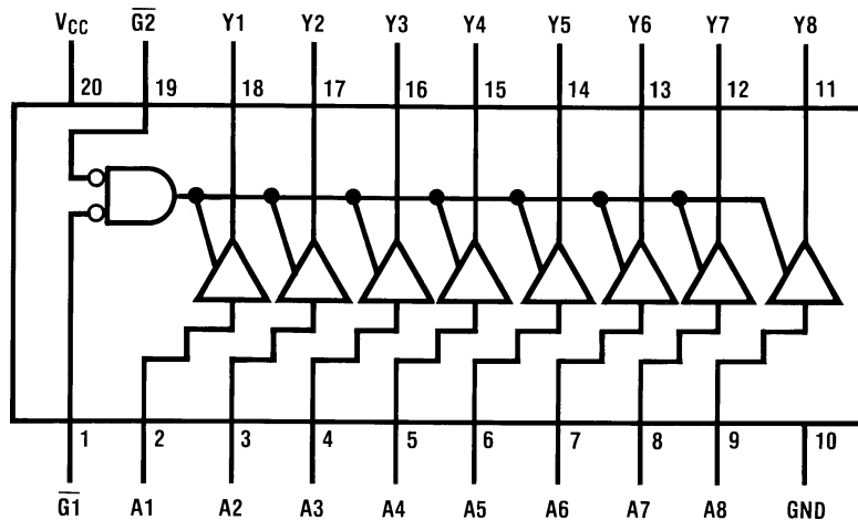
Top View, MM74HCT541
