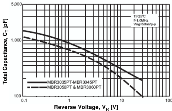
Figure 5. Total Capacitance
