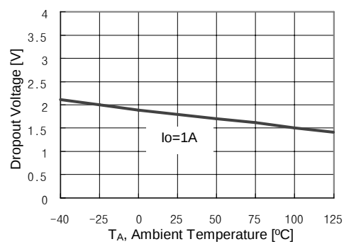
Figure 4. Dropout Voltage
