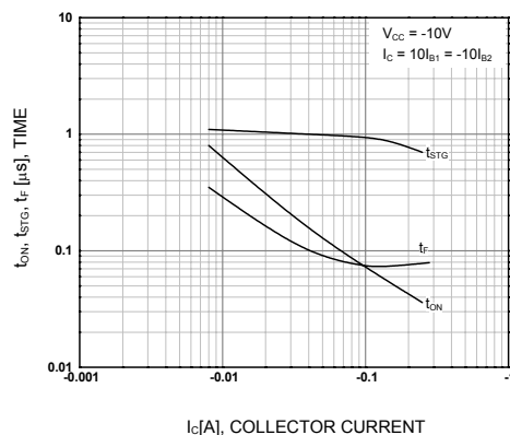
Figure 6. Switching Time
