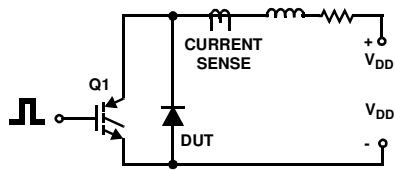
Figure 13. Avalanche Energy Test Circuit
