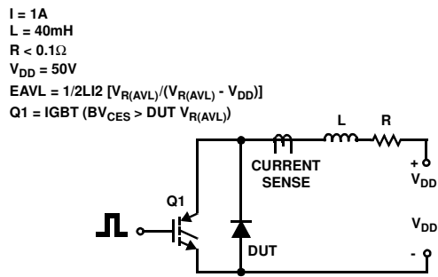
Figure 13. Avalanche Energy Test Circuit
