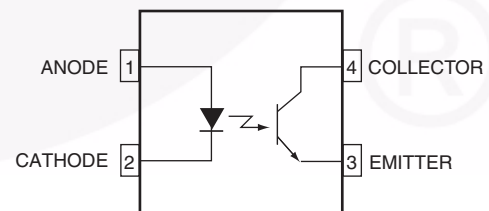
Equivalent Circuit
