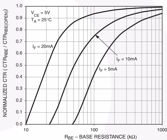
Fig. 4 CTR vs. R_{BE} (Unsaturated)
