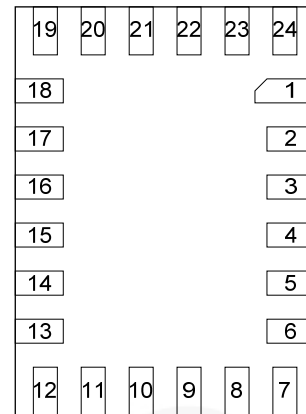
Figure 3. Bottom View
