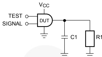
Figure 4. Test Circuit
