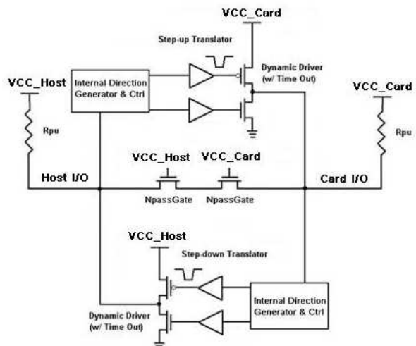
Figure 12. I/O Pin Functional Diagram
