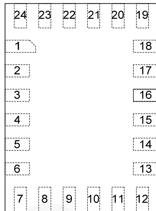
Figure 2. Top Through View
