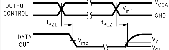
Figure 4. 3-State Output Low Enable and Disable for Low Voltage Logic
