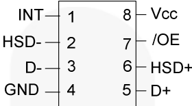
Figure 3. US8 (Top Through View)
