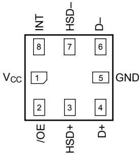
Figure 4. UMLP (Top Through View)
