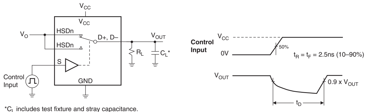
Figure 10. Break-Before-Make ( t_{BBM} )
