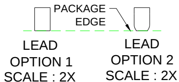
Figure 20. 10-Lead, Quad, Ultrathin Molded Leadless Package (UMLP), 1.4 x 1.8mm
