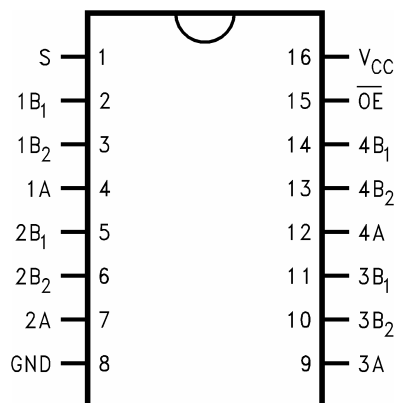
Figure 2. Connection Diagram
