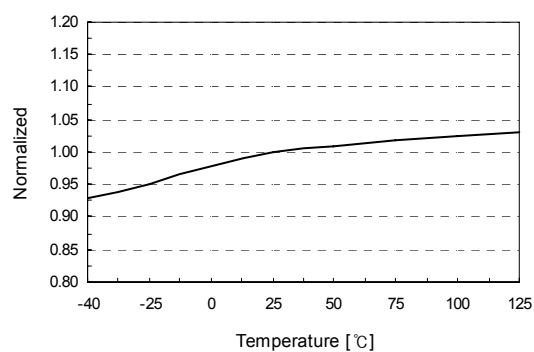
Figure 11. Shutdown Delay Current ( I_{DELAY} ) vs. T_A
