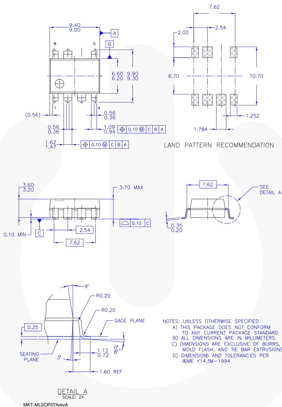
Figure 23. 7-Lead, MLSOP
