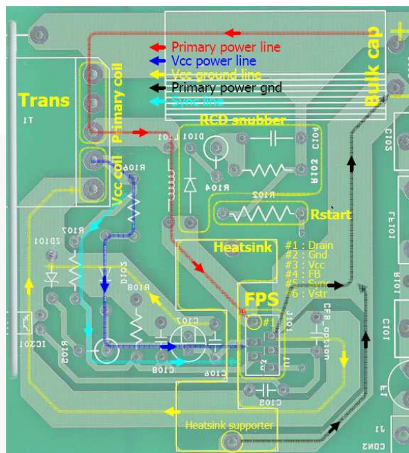
Figure 37. Recommended PCB Layout
