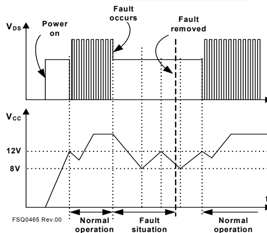
Figure 28. Auto Restart Protection Waveforms
