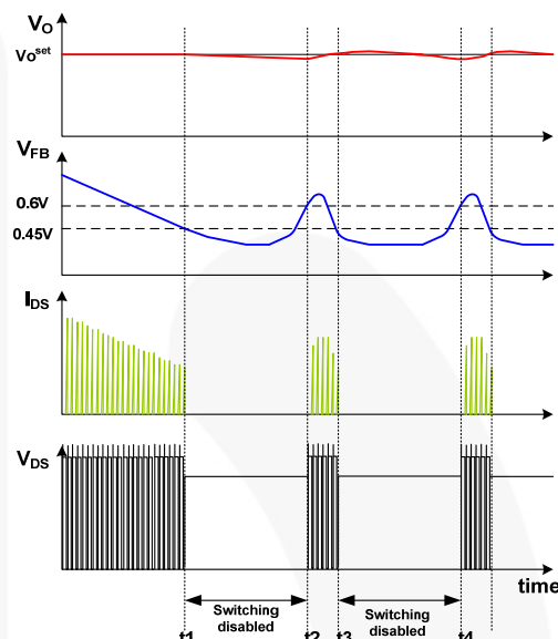
Figure 22. Burst-Mode Operation
