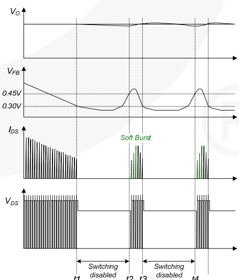
Figure 25. Burst-Mode Operation
