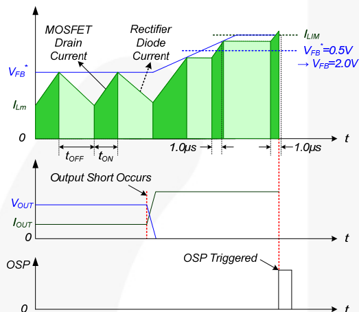
Figure 23. Output-Short Protection
