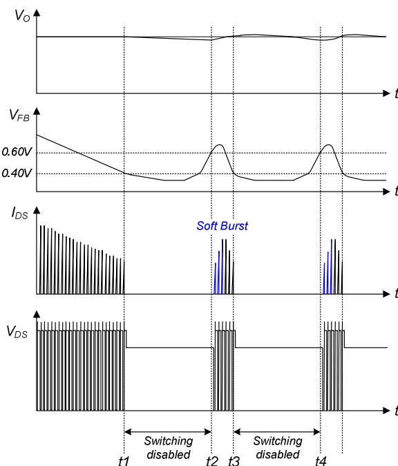
Figure 23. Burst-Mode Operation
