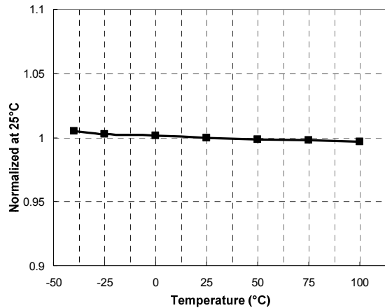
Figure 9. Low-Side V_{CC} ( LV_{CC} ) Stop vs. Temperature
