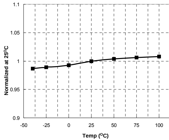
Figure 11. V_{RT} Voltage vs. Temperature
