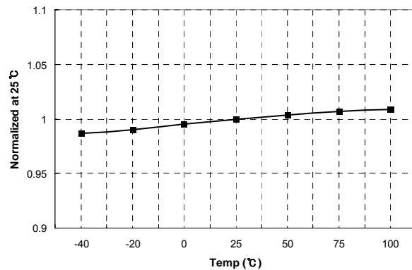
Figure 15. V BH Voltage vs. Temperature
