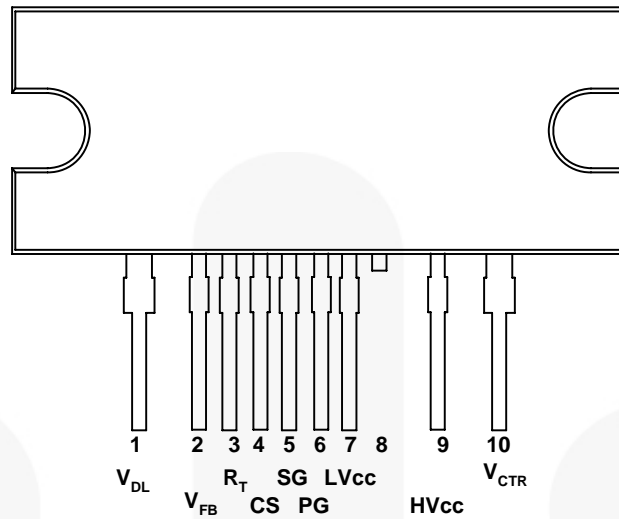
Figure 4. Package Diagram
