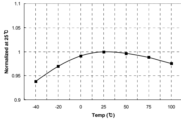
Figure 11. OLP Delay Current vs. Temperature
