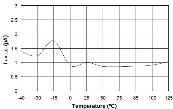
Figure 21. Leakage Current after Startup ( I_{HV-LC} ) vs. Temperature
