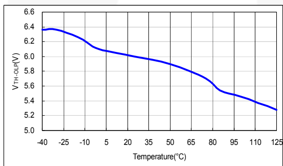
Figure 10. V_{TH-OLP} vs. Temperature
