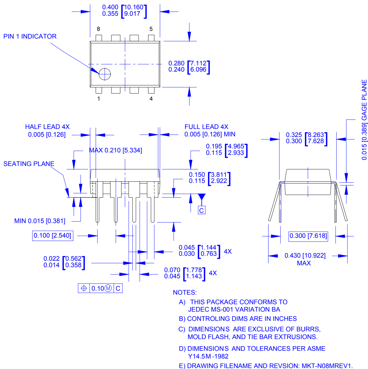
Figure 30. 8-Pin Dual In-Line Package (DIP)
