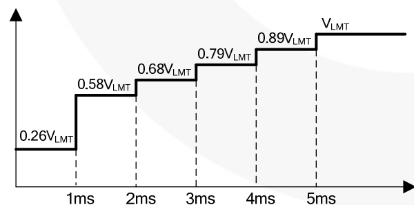
Figure 23. Soft-Start Function
