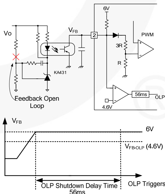
Figure 29. OLP Operation
