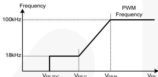
Figure 26. PWM Frequency
