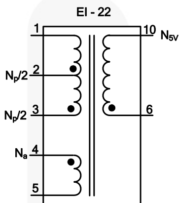
Figure 30. Transformer Specification
