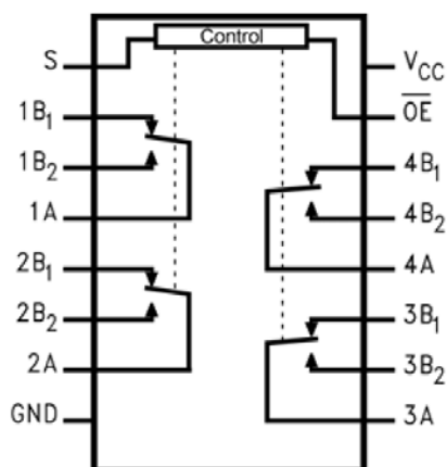
Figure 2. Analog Symbol
