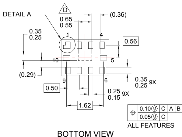
Figure 18. 10-Lead, MicroPak™ 1.6 x 2.1mm JEDEC MO255B
