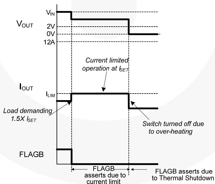
Figure 29. OUT Overloaded with 1.5X I_{LIM} (Long-Duration Overload)
