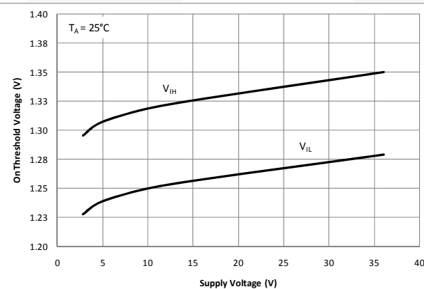
Figure 13. ON Threshold vs. Supply
