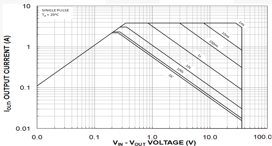
Figure 40. FPF2702 MX SOA
