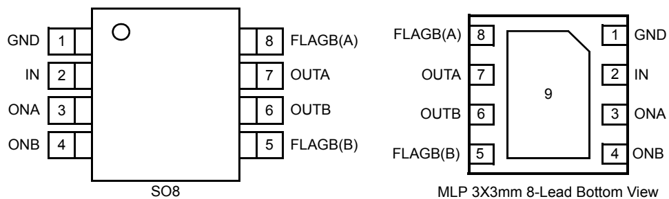
Figure 5. Pin Configurations
