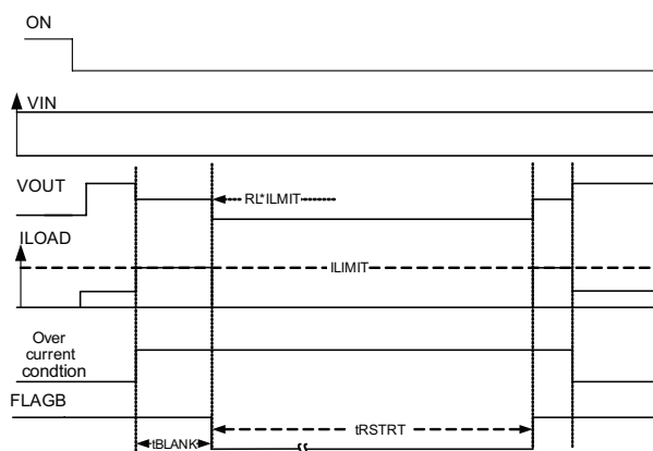
Figure 36. FPF2300 FLAGB Reports While Entering into an Over-Current Condition
