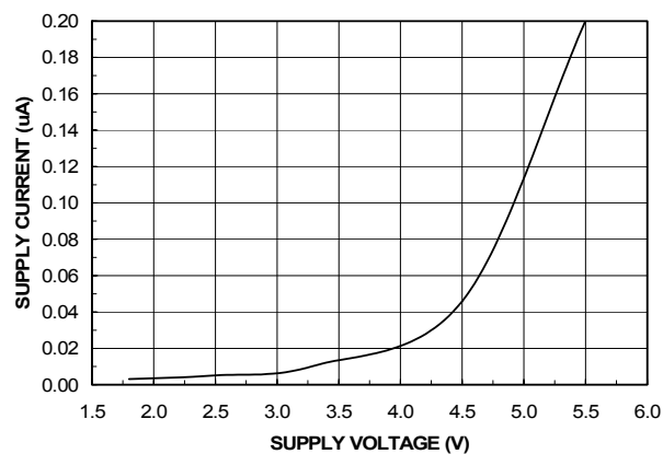
Figure 5. Reverse Current vs. V_{\text{OUT}}
