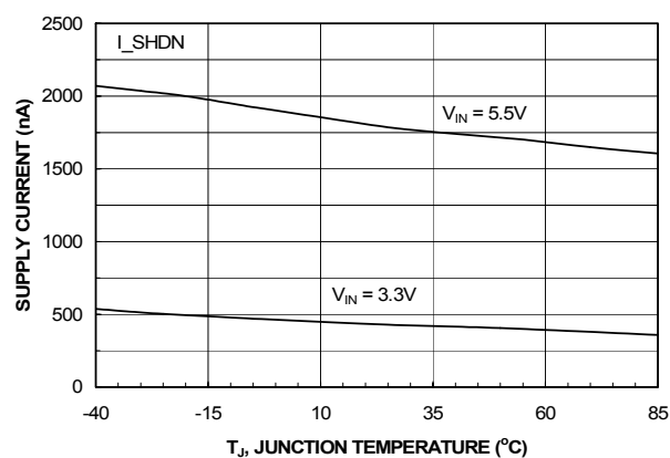
Figure 3. I_{\text{SHUTDOWN}} Current vs. Temperature
