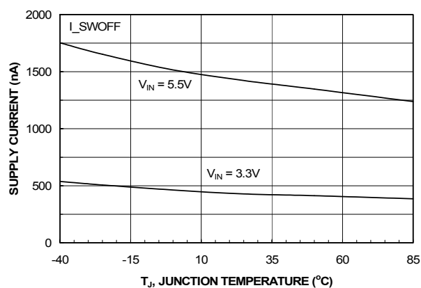
Figure 4. I_{\text{SWITCH-OFF}} Current vs. Temperature
