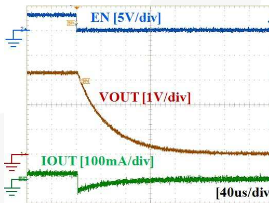
Figure 29. Turn-Off Response with FPF1321 (VIN=3.3V, CIN=1μF, COUT=1μF, RL=150Ω, SEL=LOW)
