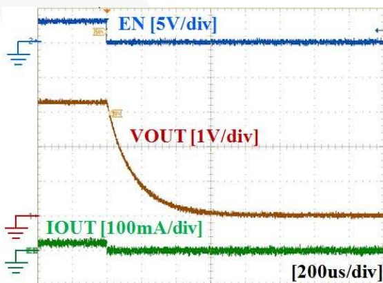
Figure 28. Turn-Off Response with FPF1320 (VIN=3.3V, CIN=1μF, COUT=1μF, RL=150Ω, SEL=LOW)
