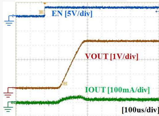
Figure 27. Turn-On Response (VIN=3.3V, CIN=1μF, COUT=1μF, RL=150Ω, SEL=LO)
