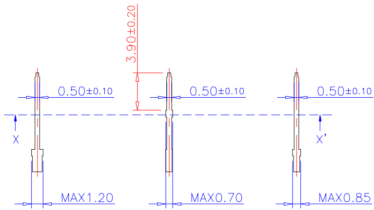
LEAD TYPE 1
