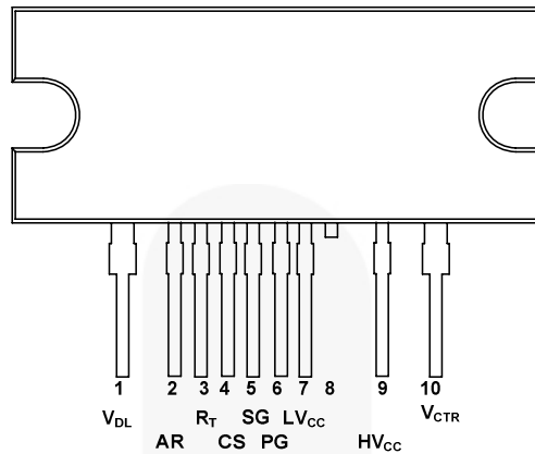
Figure 3. Package Diagram
