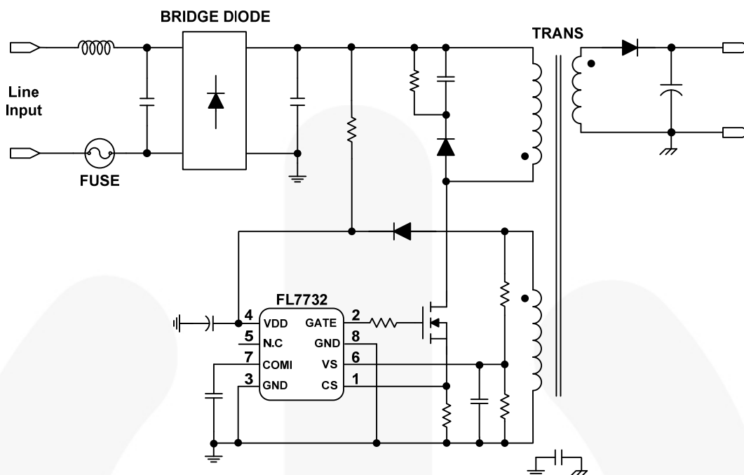
Figure 1. Typical Application
