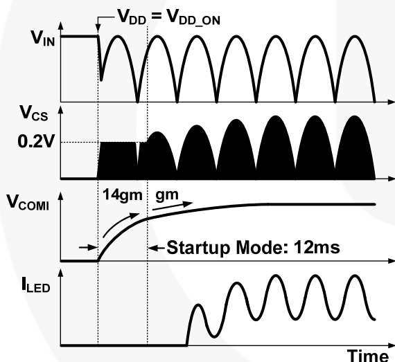
Figure 15. Startup Sequence
