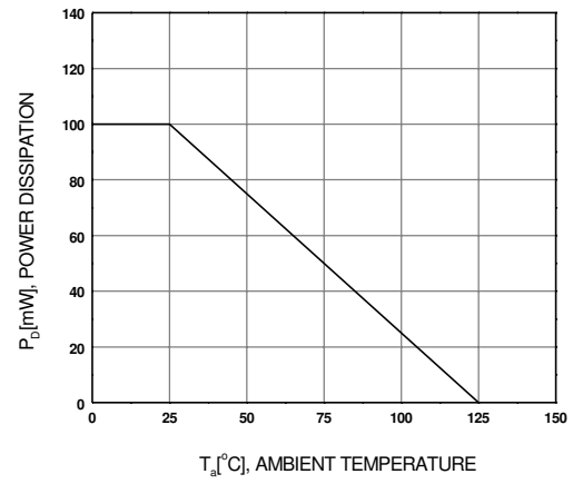
Figure 8. P_D - T_A
