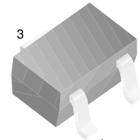
1 SOT-323 Marking: SCH 1. Drain 2. Source 3. Gate
