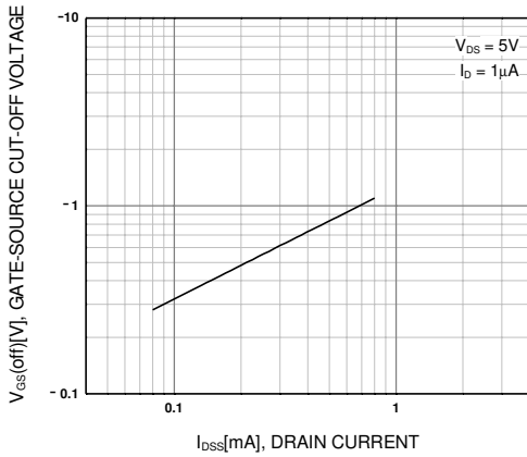
Figure 5. V_{GS(off)} - I_{DSS}
