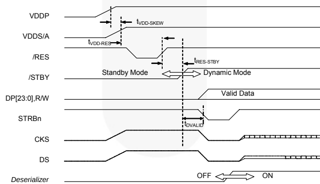
Figure 18. Power-Up Timing
