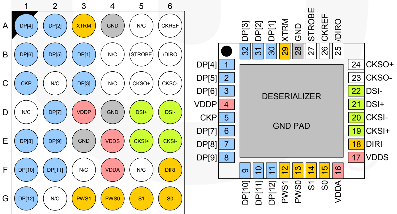
42-Ball BGA, 3.5 x 4.5mm, .5mm pitch (Top View)
