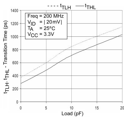
FIGURE 19. Transition Time vs. Load
